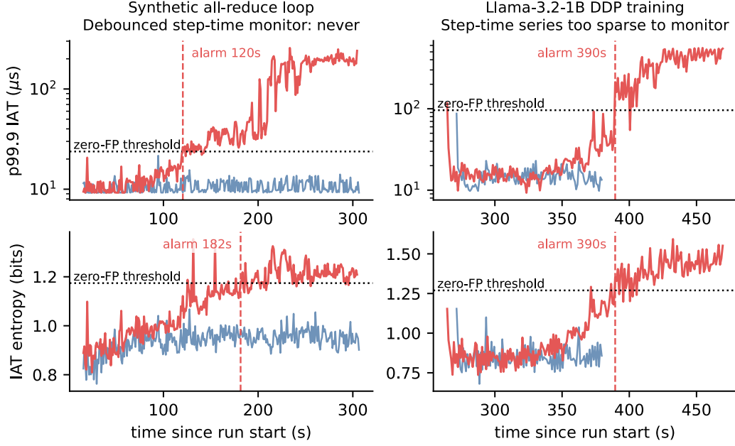
Figure 4. The endpoint statistics alarm where the production monitors are silent. Entropy and the p99.9 tail over time, healthy against a matched flooded run. Left: a synthetic all-reduce loop, where a debounced step-time monitor never trips. Right: real Llama-3.2-1B training, where the two statistics detect the flood with zero false alarm before onset while the step-time series is too sparse to threshold.
