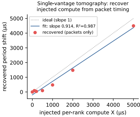
Figure 5. One endpoint recovers the compute magnitude. Recovered against injected extra compute on real hardware, with the ideal line. The fit has slope 0.914 and R^2 = 0.987 .
