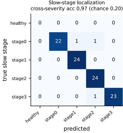
Figure 6. Endpoint timing names the slow stage on unseen severities. Confusion matrix for four pipeline stages plus a healthy class, trained on one set of severities and tested on another. Accuracy is 0.97 against a chance rate of 0.20.
